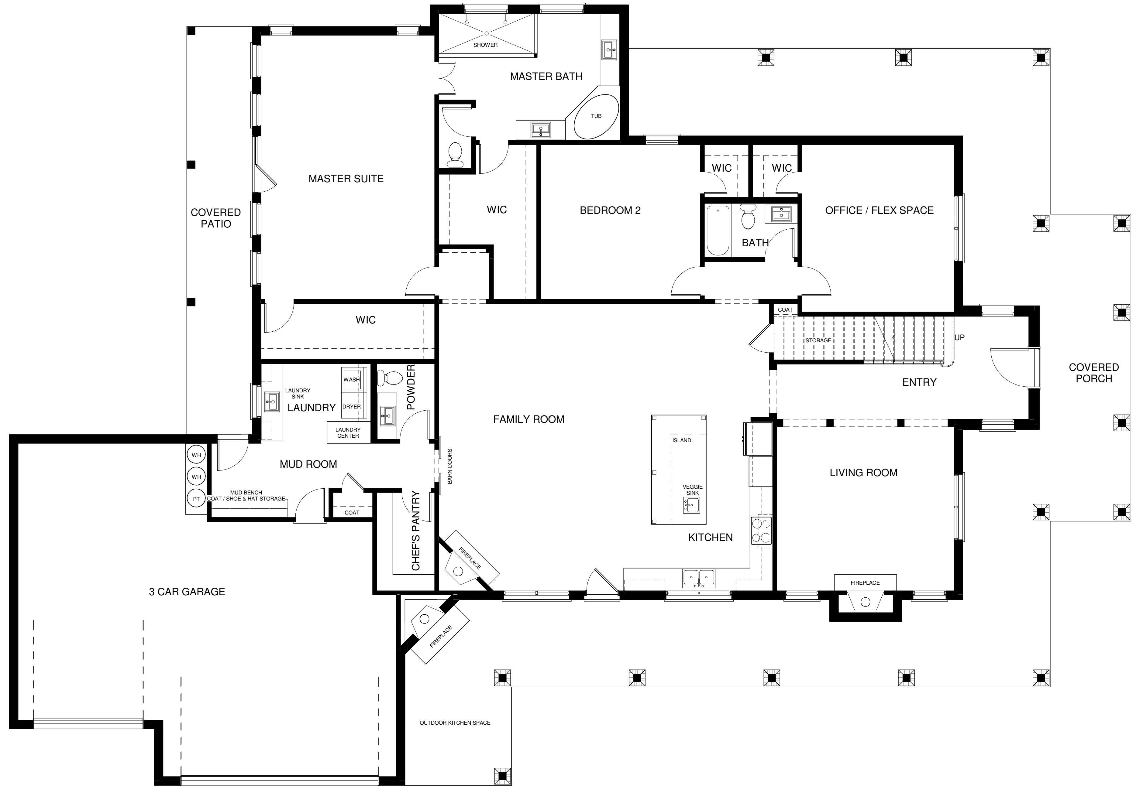
1 FLOOR PLAN 1ST SALES 3/16" = 1'-0"
